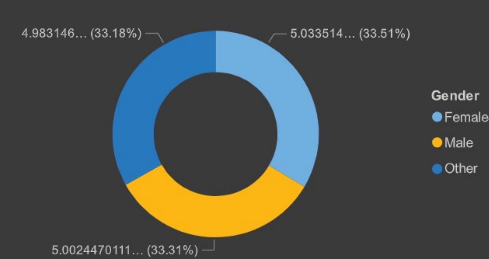
Survival by Gender
