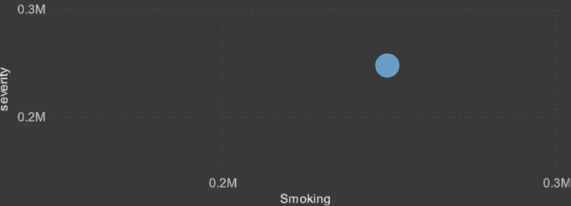
Smoking vs Severity
