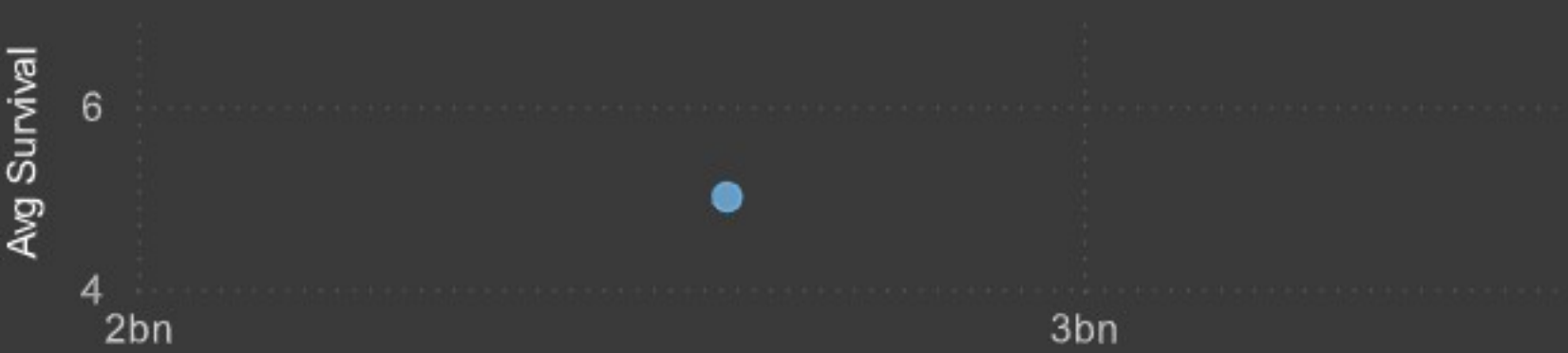
Treatment by Cost bySurvival
