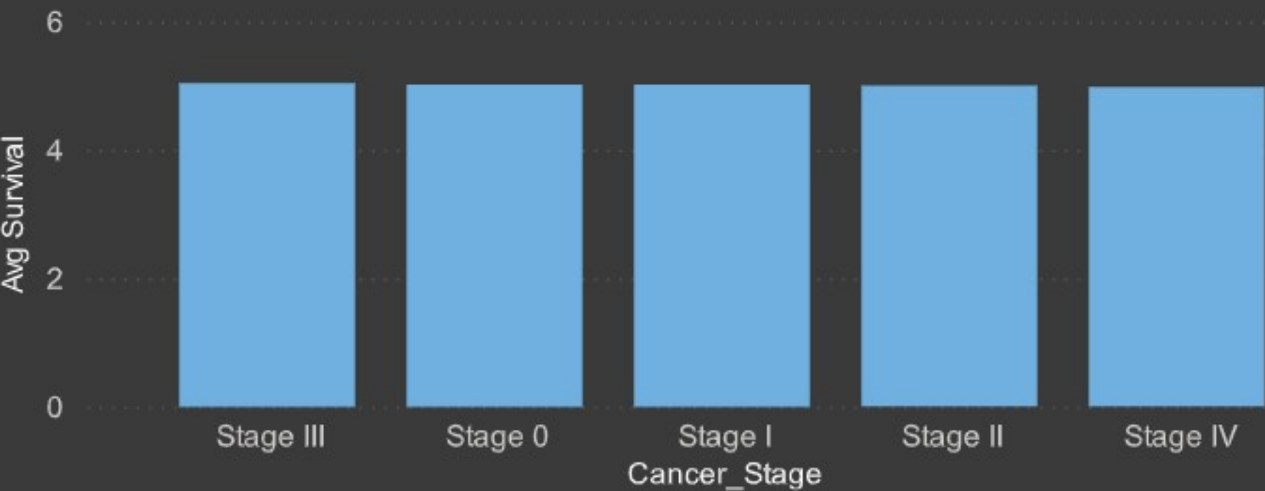
Survival by Stage
